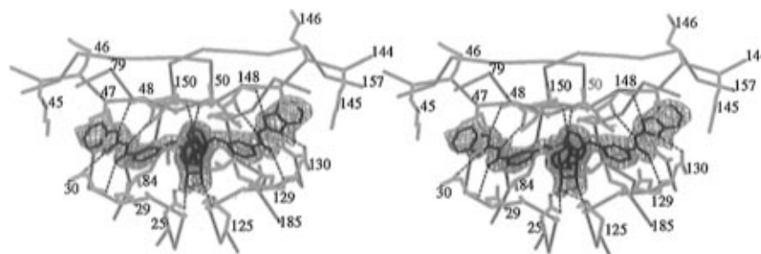
Figure 3. SD146 bound in the active site of HIV PR. The residues that interact with SD146 are drawn in blue (Table 3) and the dashed lines indicate hydrogen bonds. The C- \alpha carbons of the enzyme are drawn in red, the numbers correspond to the sequence positions of the amino acids, and a |2F_o - F_c| simulated annealed omit map of SD146 at 1.0\sigma is shown in pink.
