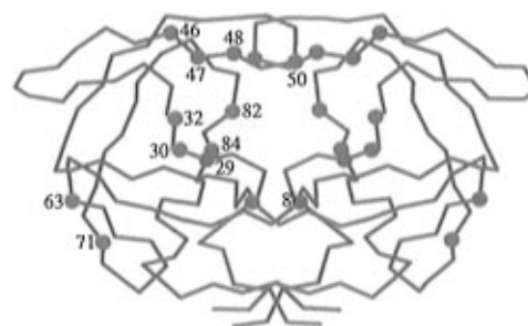
Figure 1. The C- \alpha carbon trace of HIV-1 protease complexed with the cyclic urea inhibitor SD146. The residues associated with resistance are drawn as blue circles and the numbers correspond to the sequence positions of the amino acids. The atoms of each monomer of the homodimer are drawn in red and green, and the inhibitor was omitted for clarity. The list of residues drawn in blue circles is not a complete list of known mutations.
